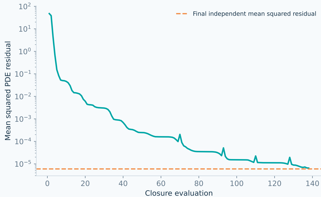
Residual minimization
